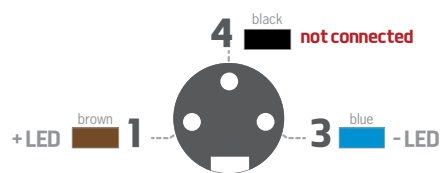
FRONT VIEW OF THE PRODUCT'S CONNECTOR
